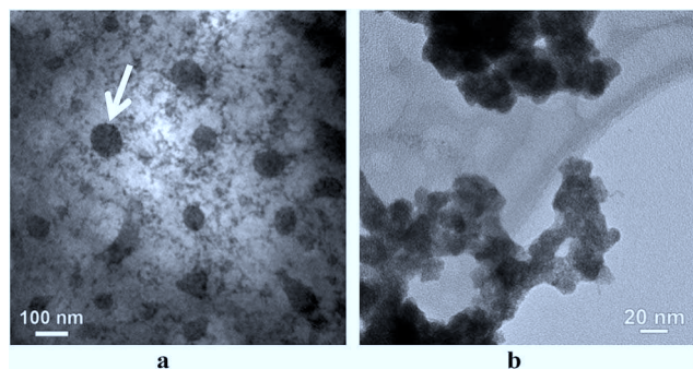
Fig. 3 TEM image of a solution of polymer GG-PIBO3 in 0.9% aqueous NaCl at 20 °C ((a), below LCST) and at 37 °C ((b), body temperature). The small diffuse entities visible across the background are uranium salt particles.
